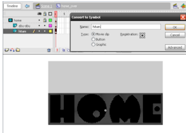
Gambar 128. Symbol Movieclip
