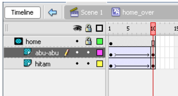
Gambar 129. Motion Tween
