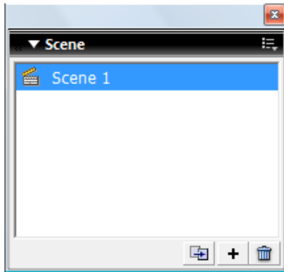
Gambar 155. Panel science
