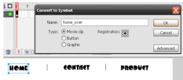
Gambar 123. Symbol Movieclip
