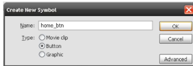
Gambar 135. Symbol button
