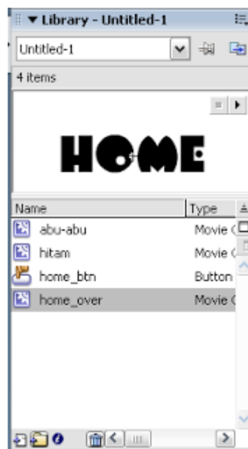
Gambar 138. Frame Over
