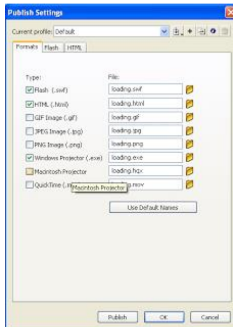
Gambar 206. Tampilan publish
