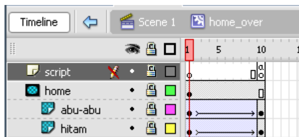
Gambar 134. Timeline
