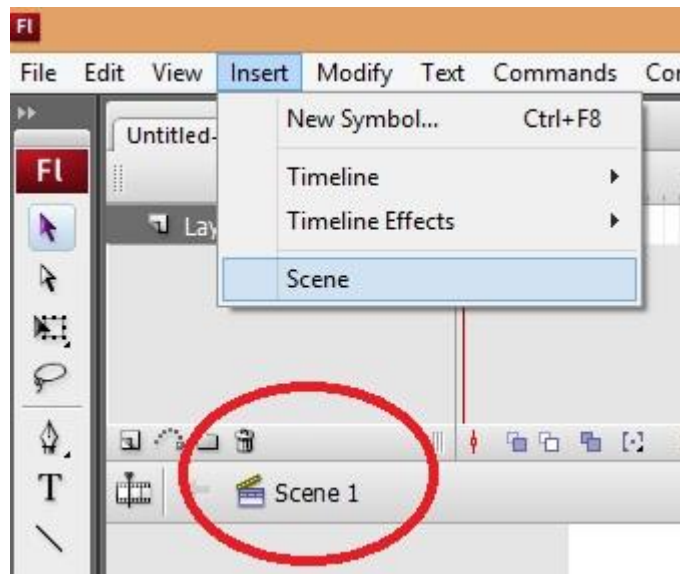
Gambar 161. Panel Science
